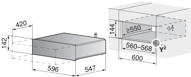
WarmingDrawer V4000 14 (34026) Built-in solo
