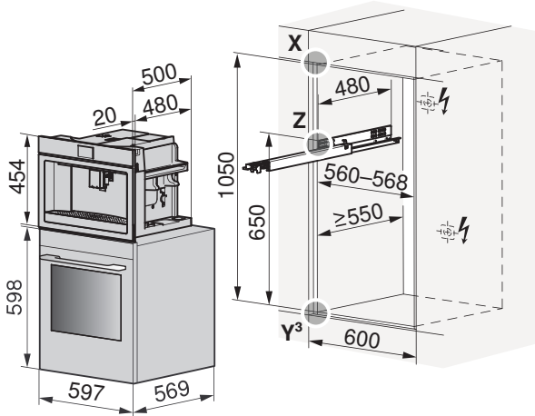
Front dimensions of the appliances: Detail X (see page 11) Internal dimension of the appliance: Detail Y 3 /Z (see page 28)
