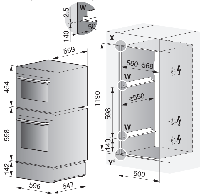
Installing with oven & compact oven or steamer
