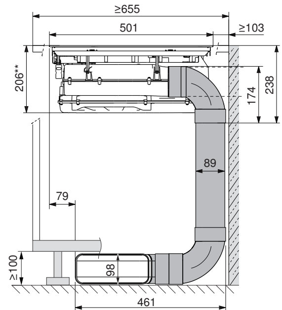
Extraction operation with flat channel system, metal
