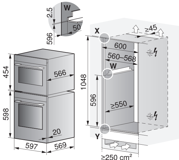
Front dimensions of the appliances: Detail X/Y (see page 11)
