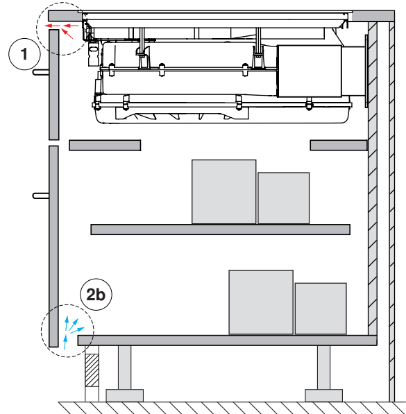
Recirculation operation without flat channel system
