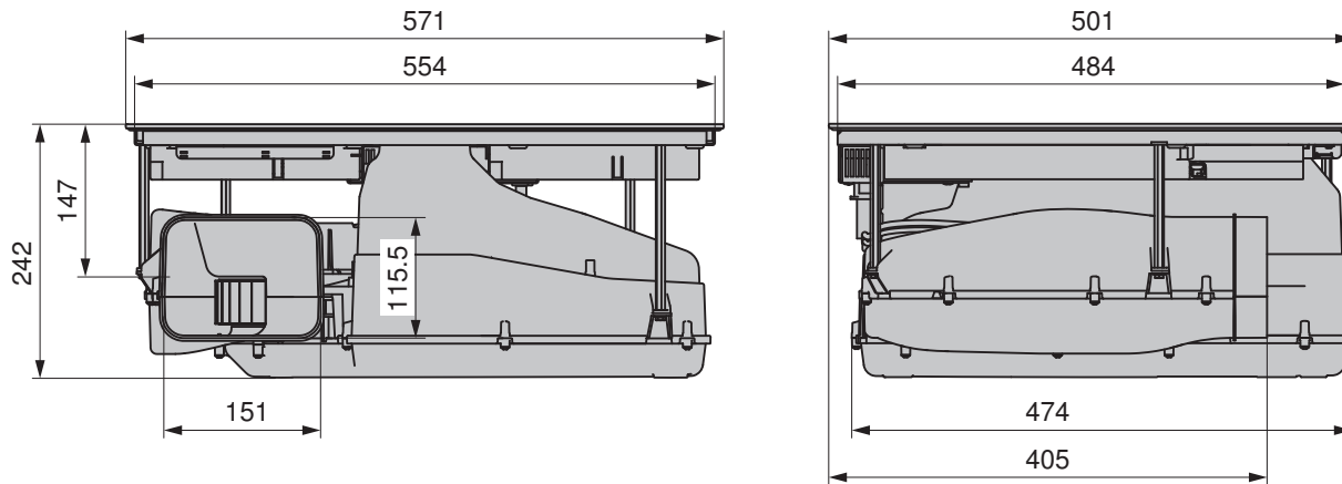
Installation for recirculation operation, unguided
