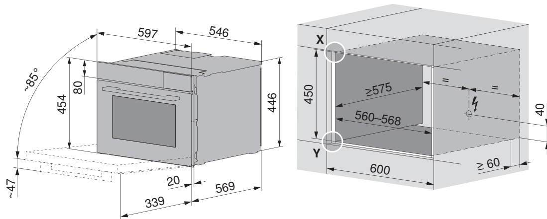
Front dimensions of the appliances: Detail X/Y (see page 11)
