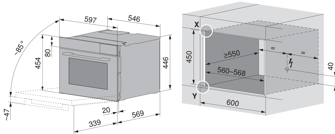
Front dimensions of the appliances: Detail X/Y
