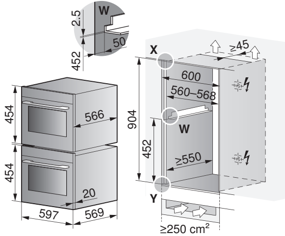
Front dimensions of the appliances: Detail X/Y (see page 11)
