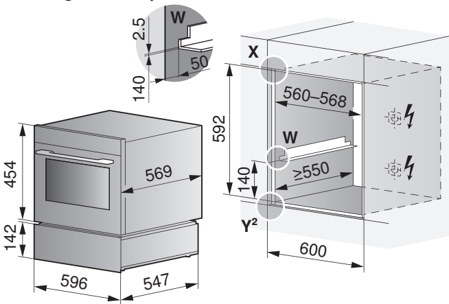
Installing with compact oven or steamer
