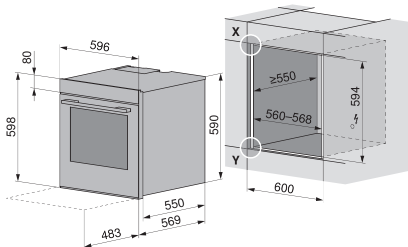
Front dimensions of the appliances: Detail X/Y
