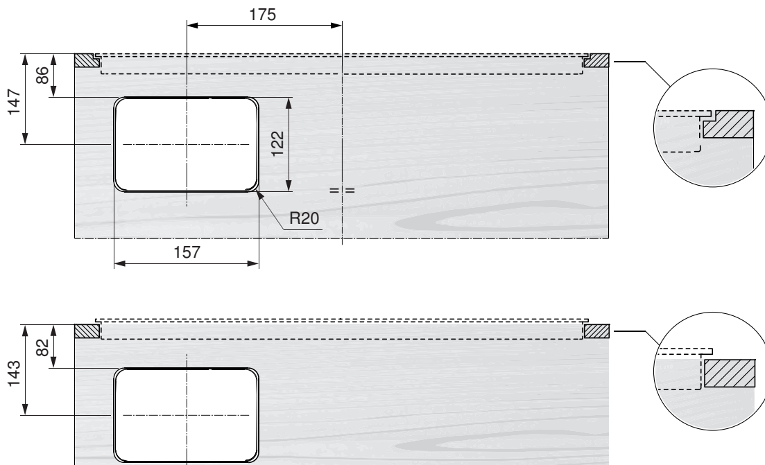
Installation for recirculation operation, unguided
