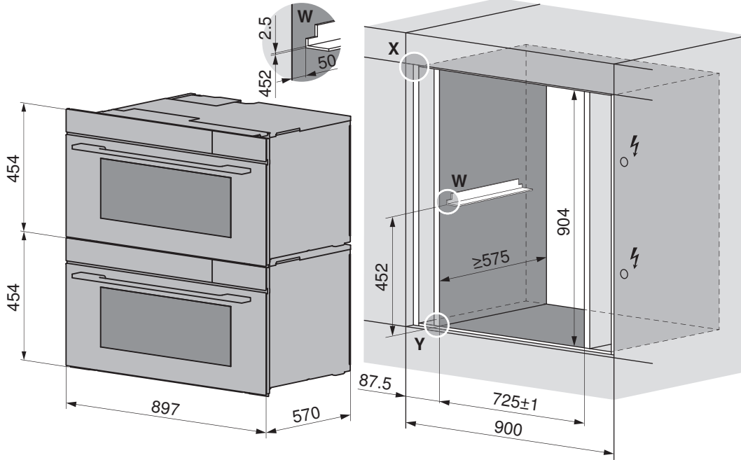
Front dimensions of the appliances: Detail X/Y (see page 11)
