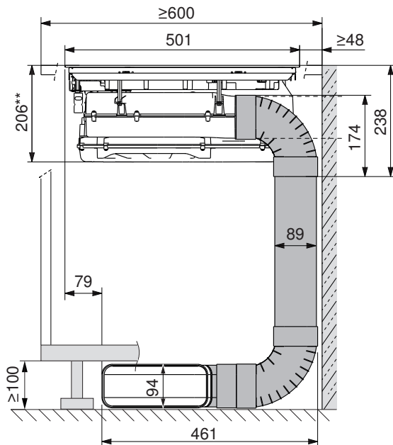
Extraction or recirculation operation with flat channel system, plastic
